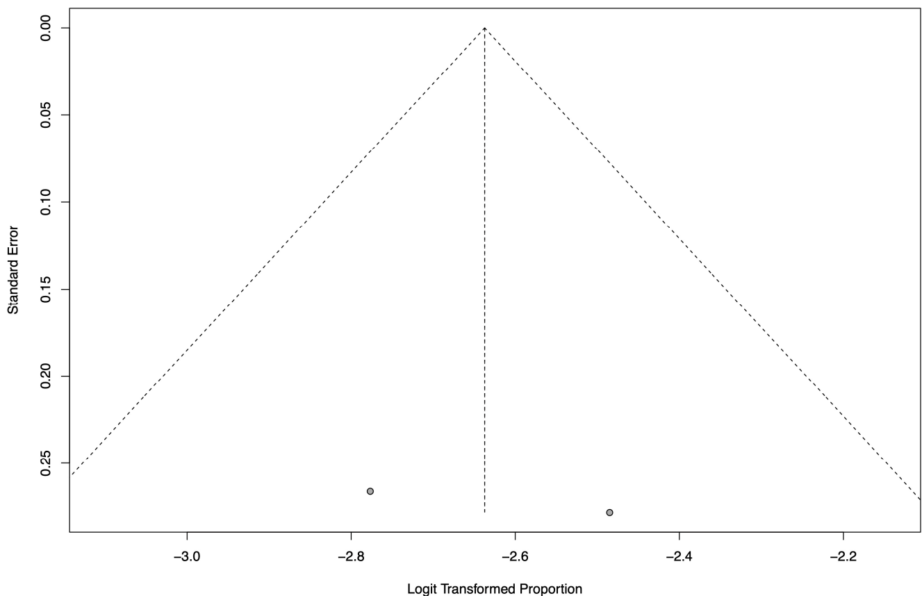
Figure 3. Meta-analysis results (all RCTs with available data) as illustrated in the forest plot and the respective funnel plot regarding the pooled prevalence estimation for COVID-19-related neuropathic pain amongst hospitalised patients [24,25].
