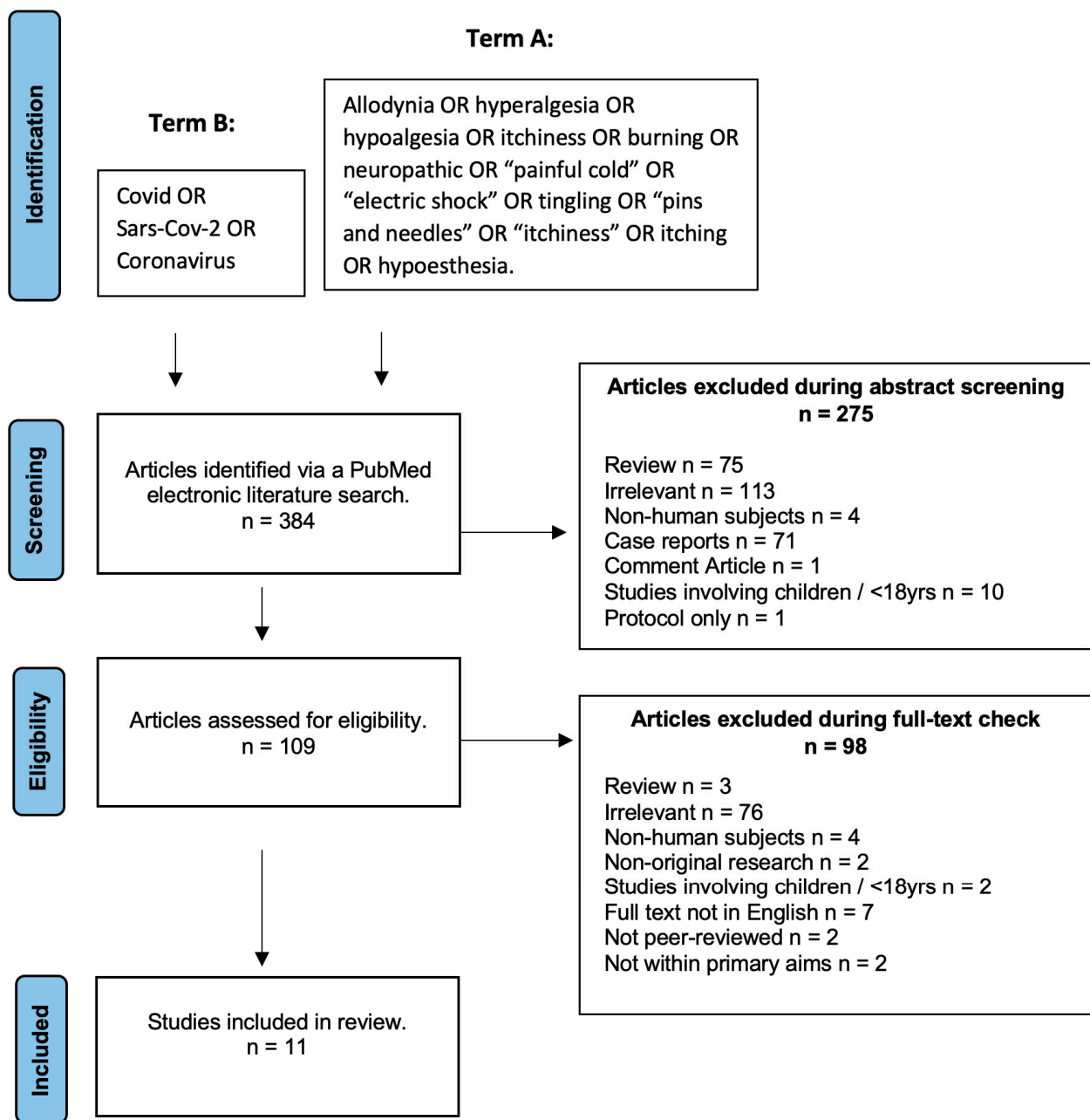
Figure 1. PRISMA chart displaying the screening and inclusion process for the COVID-19-related neuropathic pain systematic review and meta-analysis.
