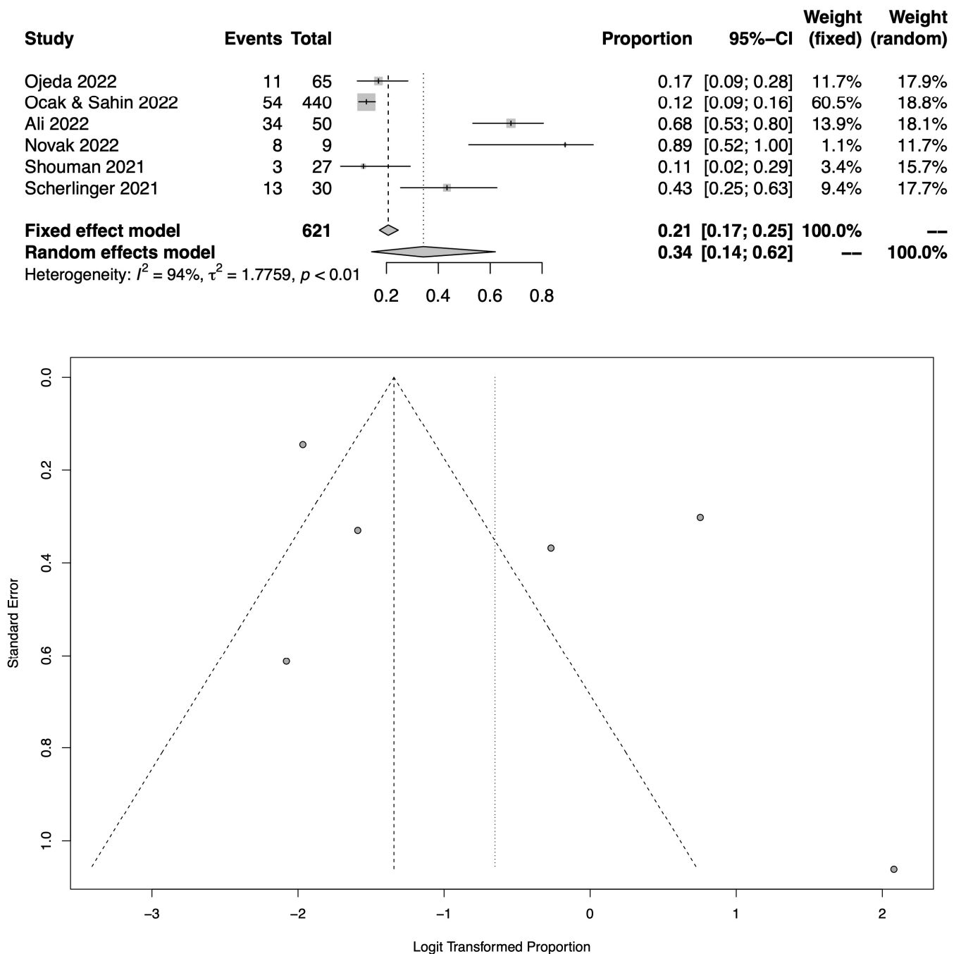
Figure 4. Meta-analysis results (all RCTs with available data) as illustrated in the forest plot and the respective funnel plot regarding the pooled prevalence estimation for COVID-19-related neuropathic pain amongst long COVID cohorts [23,26–30].
