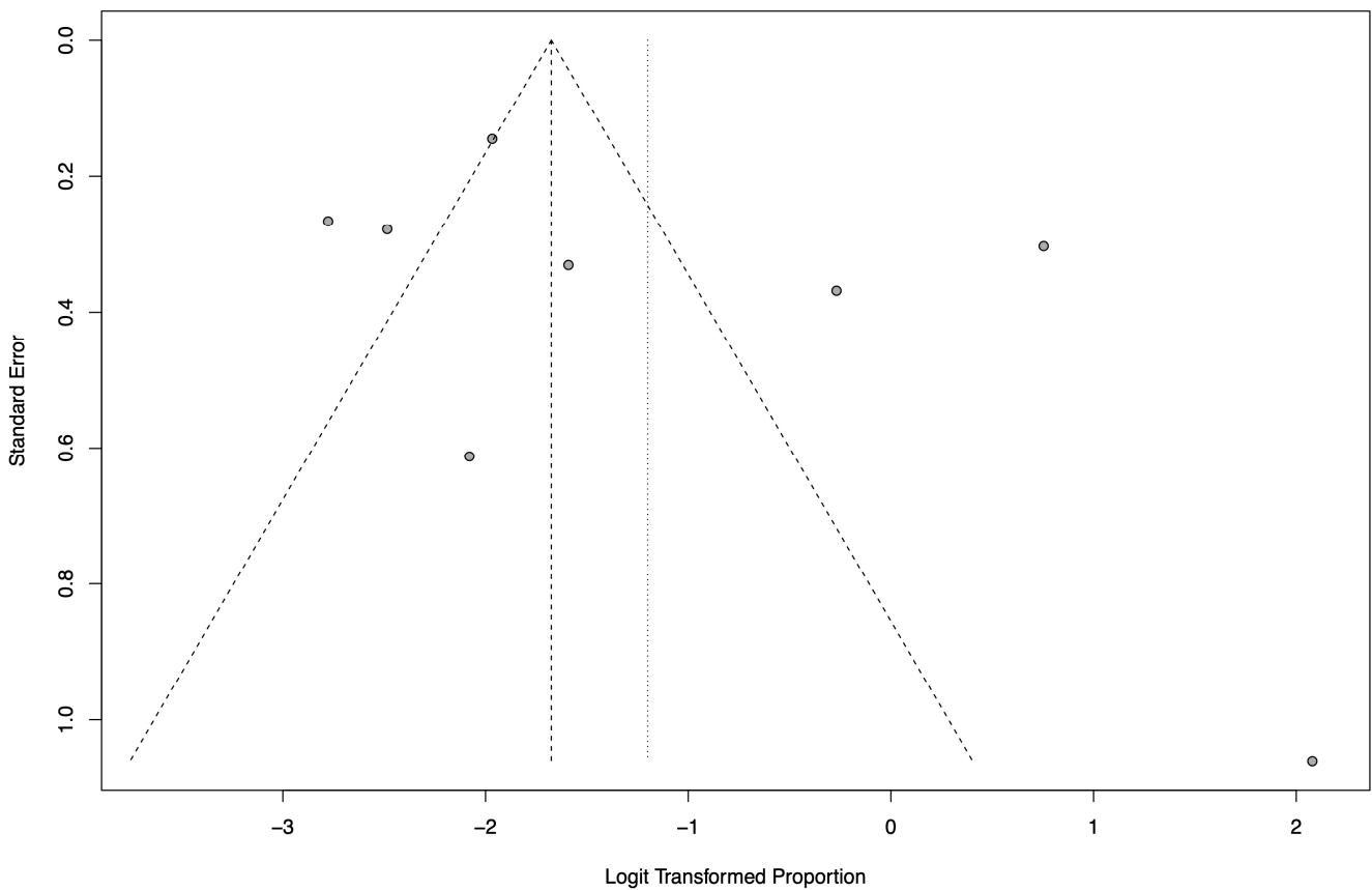
Figure 2. Meta-analysis results (all RCTs with available data) as illustrated in the forest plot and the respective funnel plot regarding the pooled prevalence estimation for COVID-19-related neuropathic pain amongst COVID-19 sufferers [23–30].
